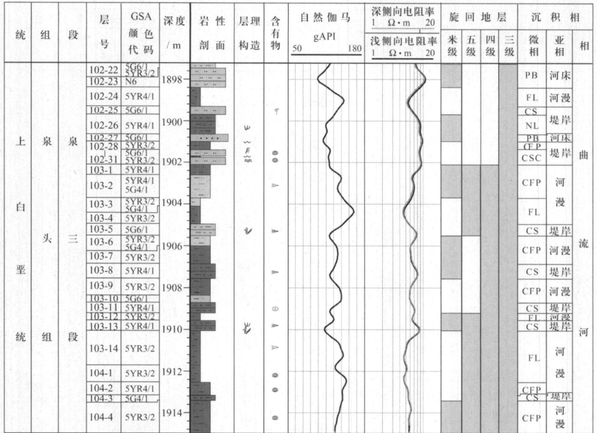
图1 松科1井南孔泉头组精细岩性-旋回地层-沉积相综合柱状图 Fig 1 Columnar section of high resolution lithology-cyclic stratigraphy and sedimentary facies of Quantou Formation (CCSD-SK 1s) *注: GSA 颜色代码系指美国地质学会颜色代码, 是国际大洋钻探岩心颜色描述通用标准 ① 。N7—浅灰色; N6—中浅灰色; N5—中灰色; N4—中深灰色; 5GY6/1—绿灰色; 5GY4/1—深绿灰色; 5G6/1—绿灰色; 5G4/1—深绿灰色; 5Y4/1—橄榄灰色; 5YR6/1—浅棕灰色; 5YR4/1—棕灰色; 5YR3/2—灰棕色 SIBB: 水下分流河道间 TS: 浊流沉积 SWOM: 静水泥水沉积 PB: 点砂坝 NL: 天然堤 CS: 决口扇 CSC: 决口水道 CFP: 河漫滩 FL: 河漫湖 ① Resources Inventory Committee. Guidelines and Standards to Terrain Mapping in British Columbia 1996. ?1994-2016 China Academic Journal Electronic Publishing House. All rights reserved. http://www.cnki.net
